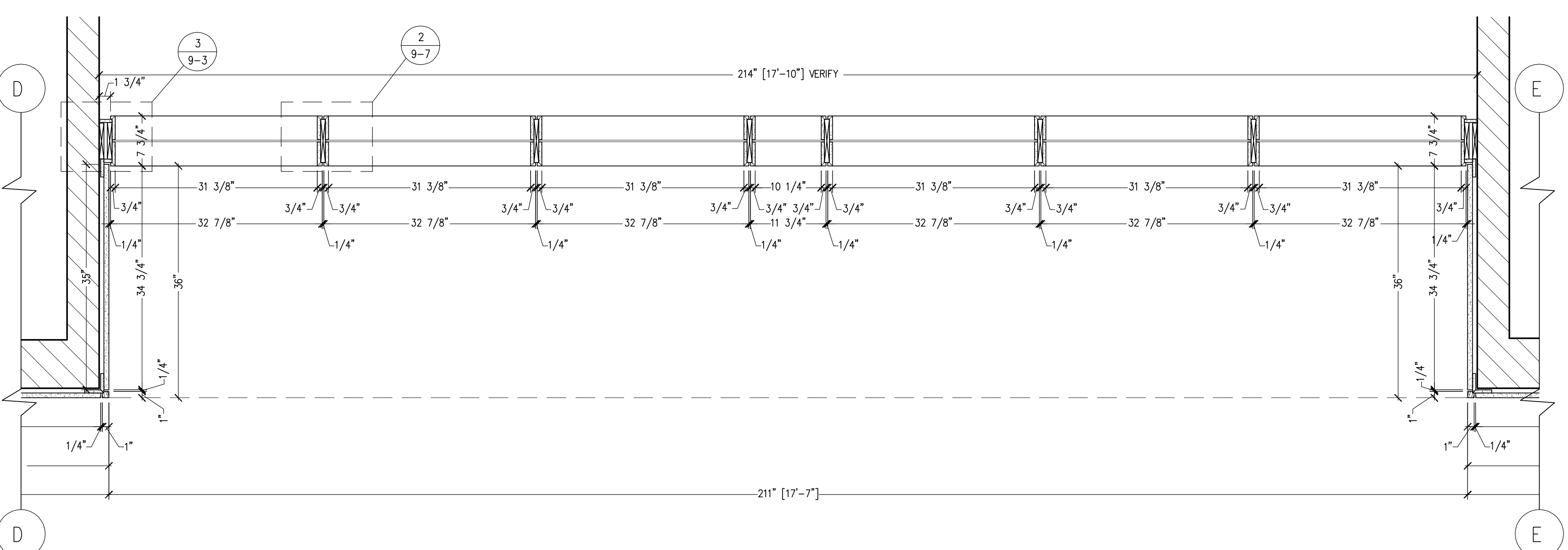
1 HORIZONTAL SECTION 9-7 SCALE: 1"=12" REF: NONE
