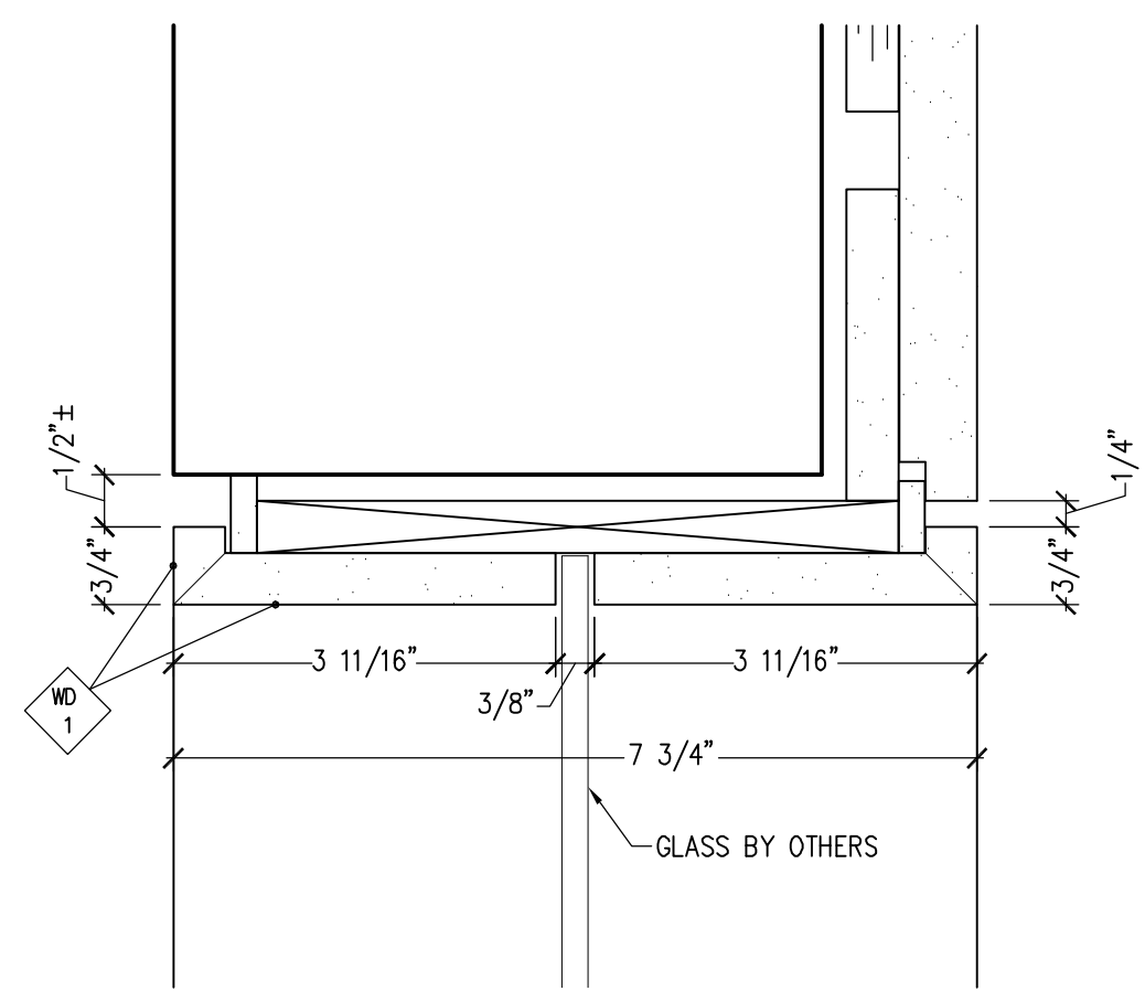
5 DETAIL 9-9 SCALE: 1 1/2"=12" REF: 15C/A-531
