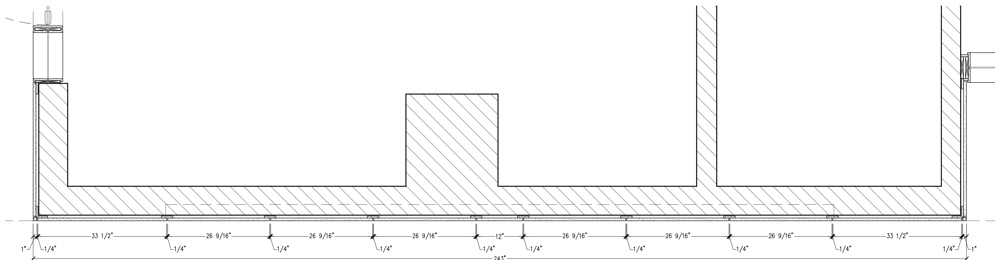
2 HORIZONTAL SECTION 9-6 SCALE: 1"=12" REF: NONE
