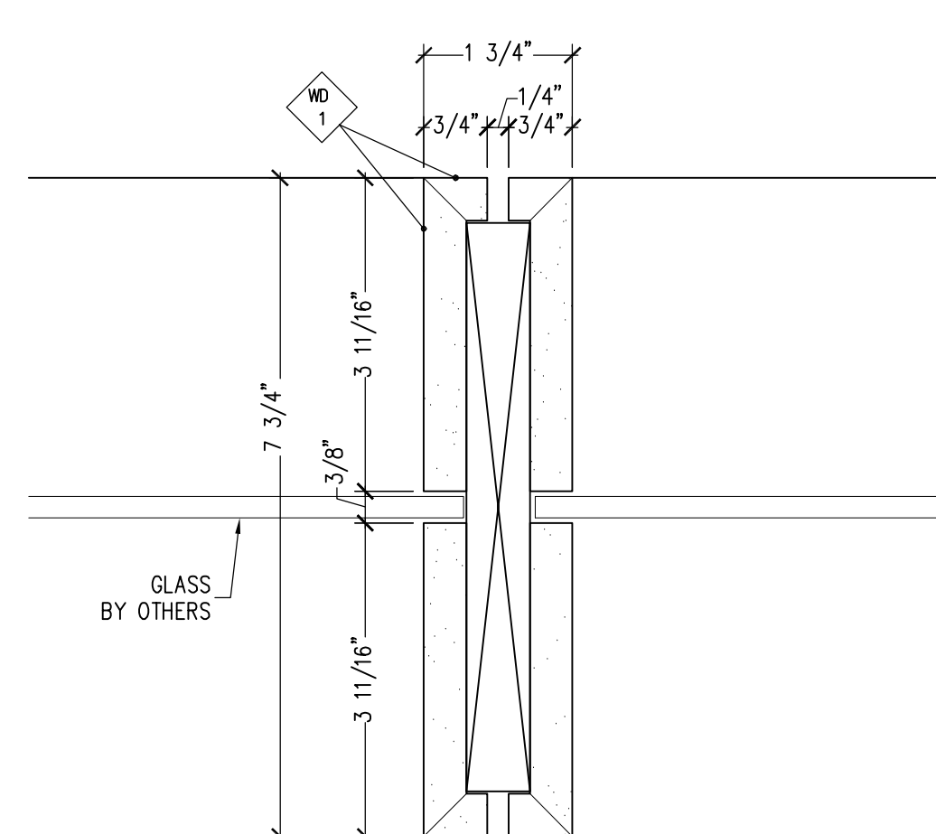
2 DETAIL 9-7 SCALE: 6"=12" REF: 15B/A-531
