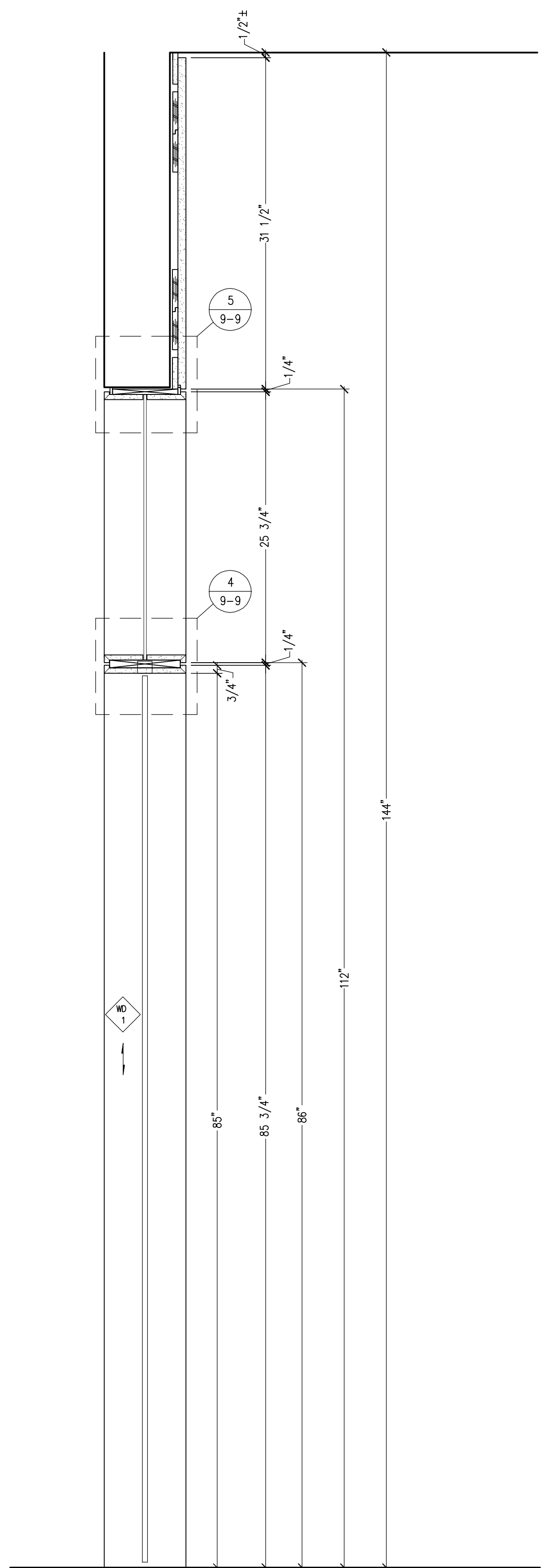
1 VERTICAL SECTION 9-9 SCALE: 1 1/2"=12" REF: NONE
