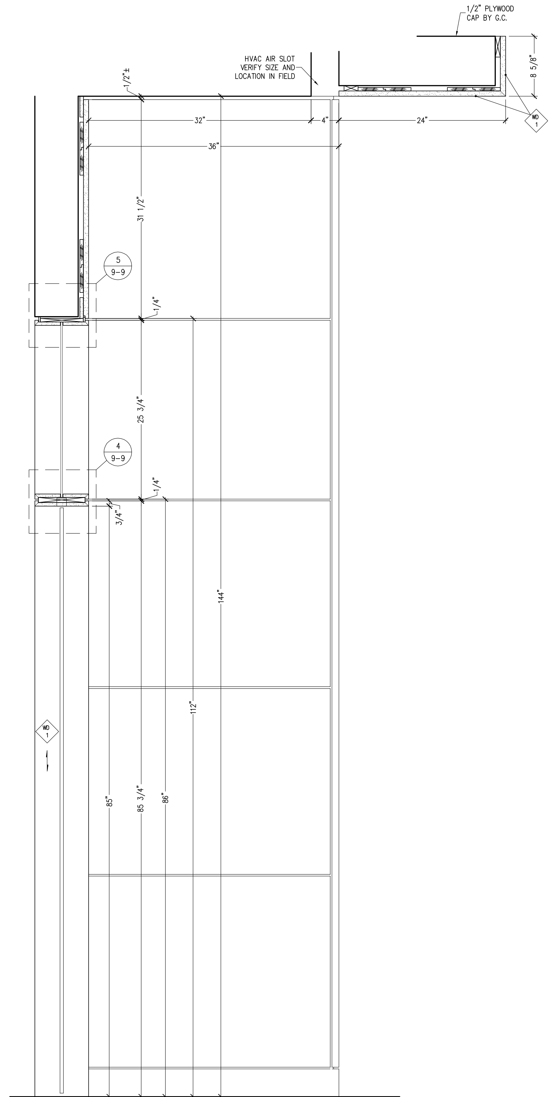
3 VERTICAL SECTION 9-9 SCALE: 1 1/2"=12" REF: NONE
