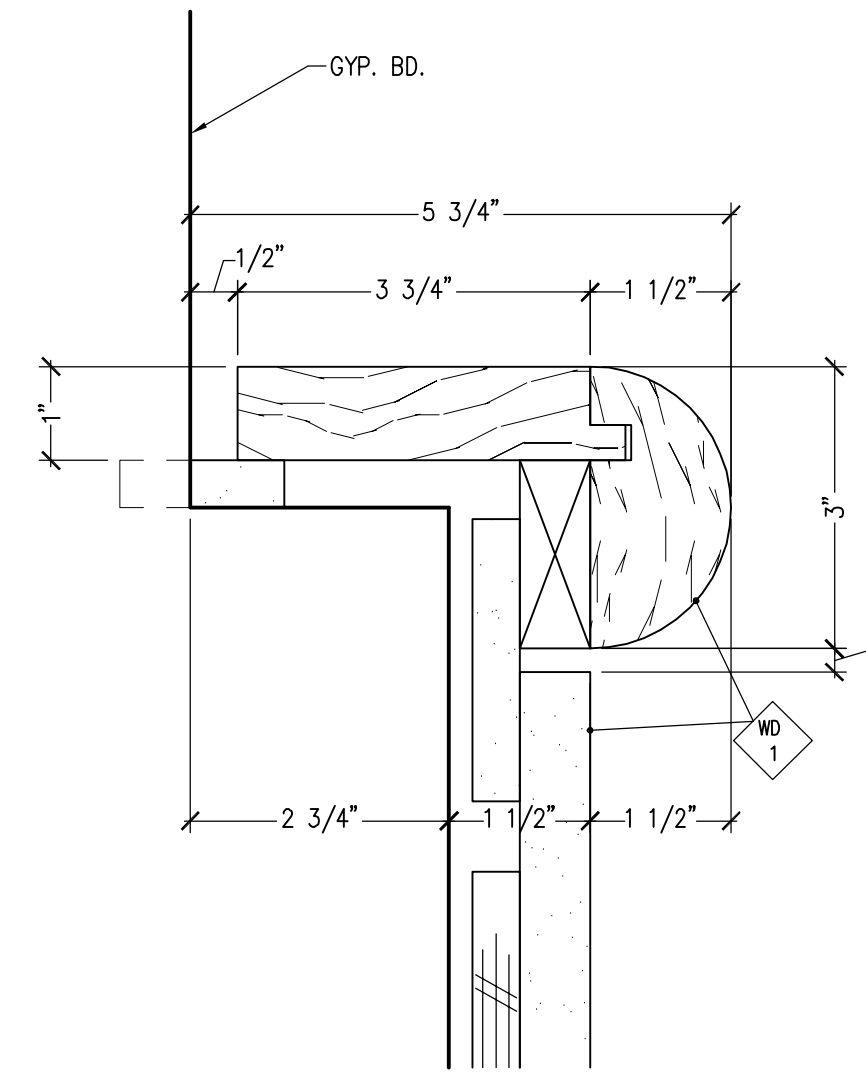
4 DETAIL 9-8 SCALE: 6"=12" REF: 3/A-531
