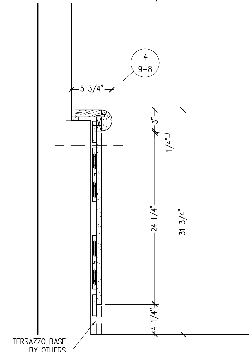
5 VERTICAL SECTION 9-8 SCALE: 1 1/2"=12" REF: 3/A-531
