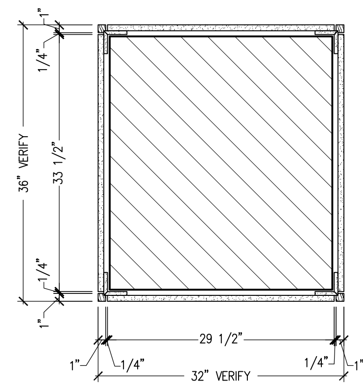
3 HORIZONTAL SECTION 9-8 SCALE: 1"=12" REF: NONE
