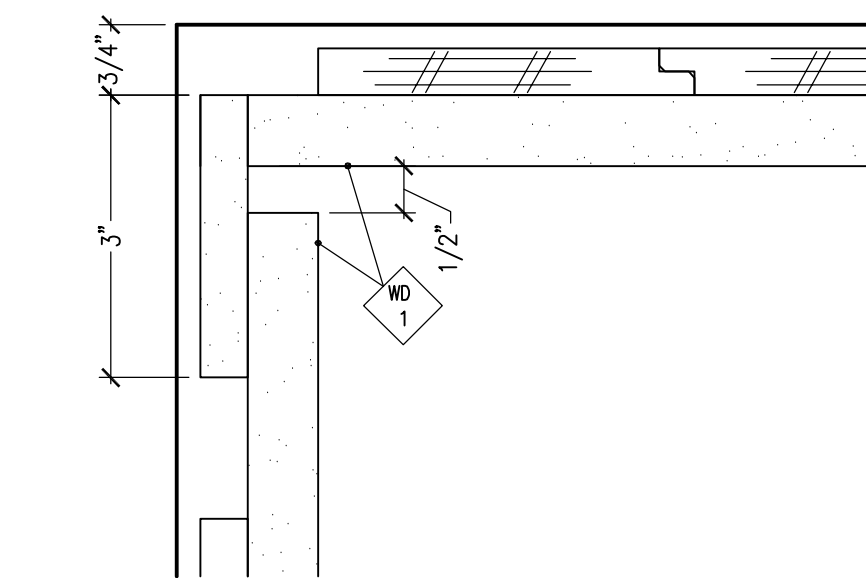
3 DETAIL 9-10 SCALE: 6"=12" REF: NONE
